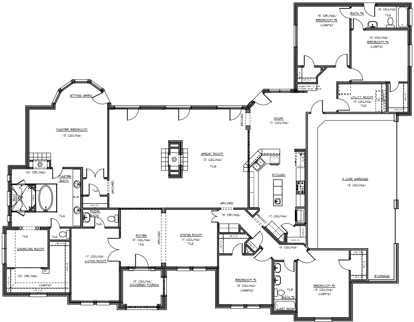
FLOOR PLAN A
