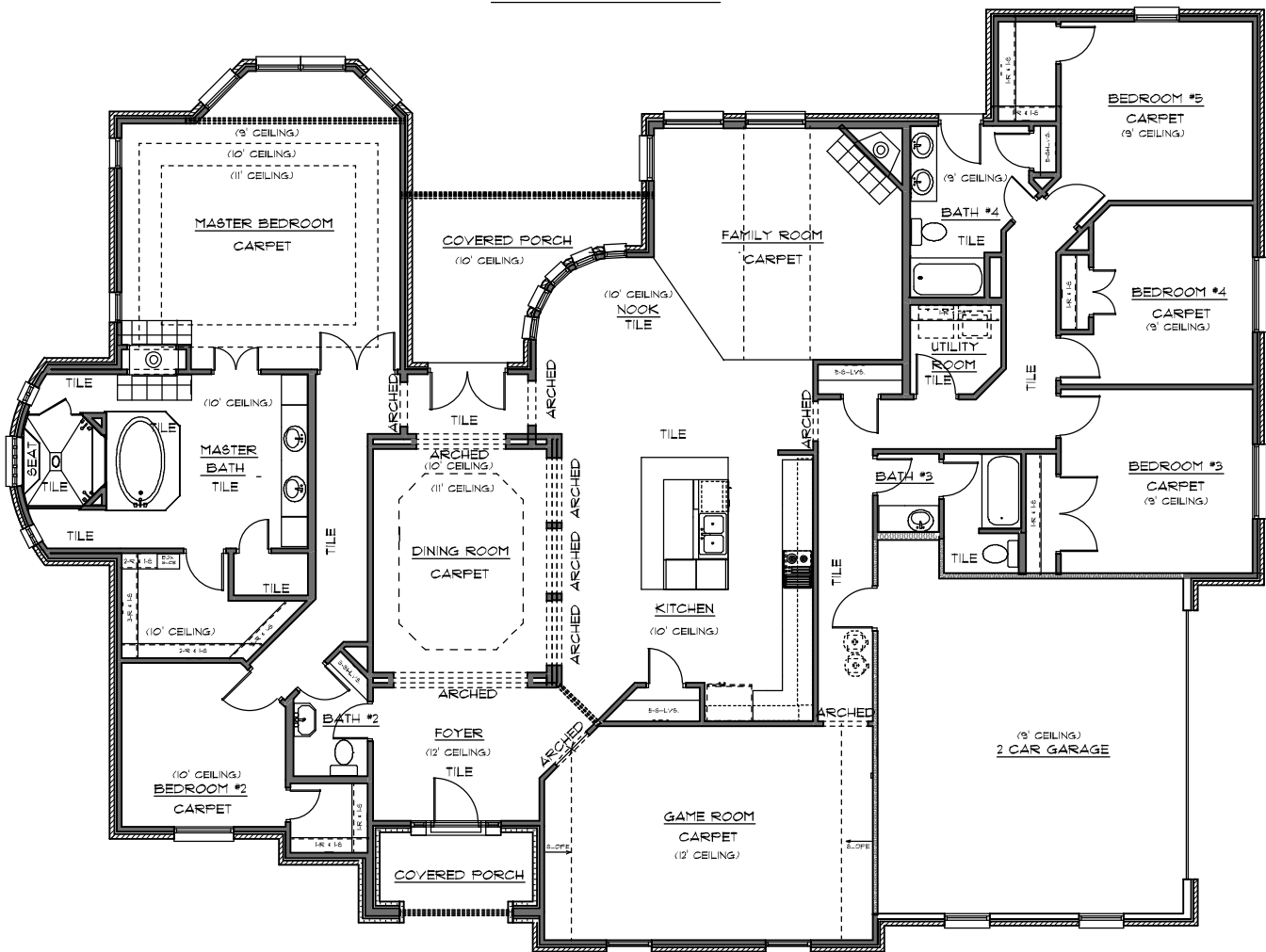
FLOOR PLAN
