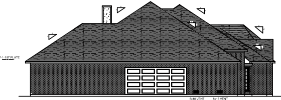
LEFT ELEVATION
