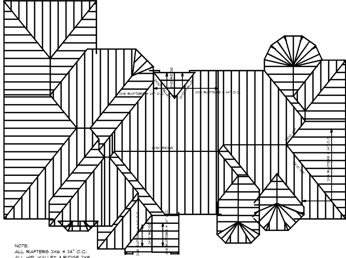
ROOF PLAN
